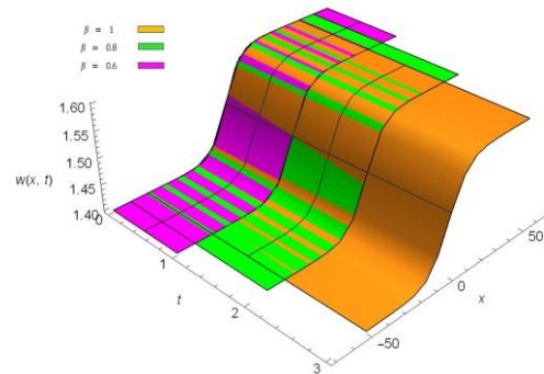
Figure 3. Surface Plot of w(x, t) for m = 0.1 , \gamma = 1.5 and various values of \beta = 0.6, 0.8, 1 with respect to t .
